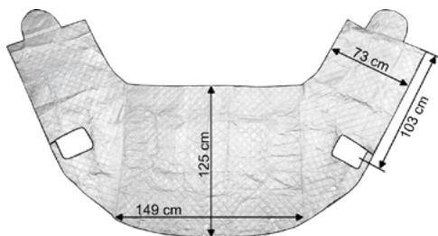
Image 1: Dimensions
