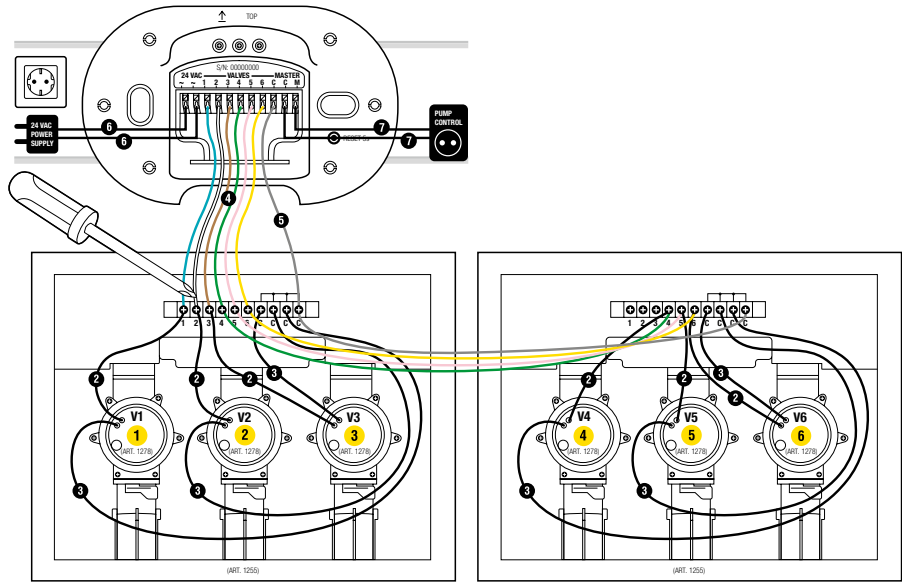
Ventilbox Art. 1255
