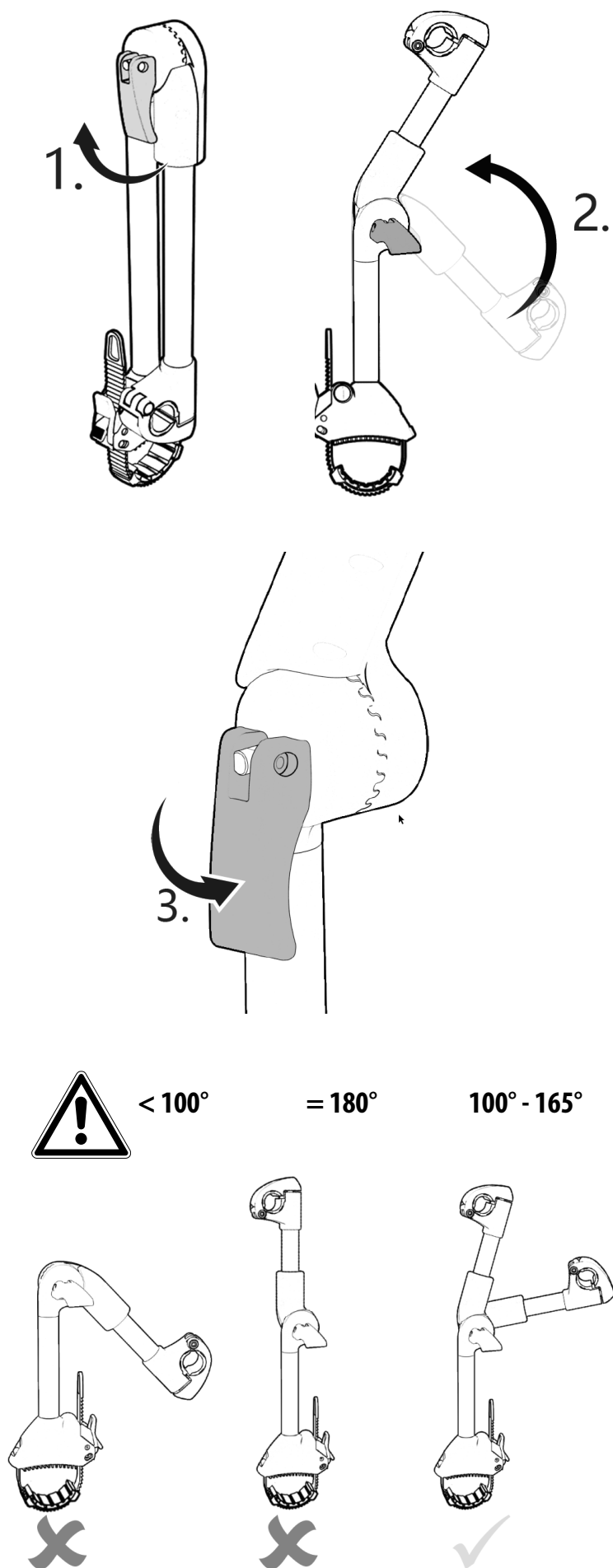
Figure 2: Folding out the frame holder
