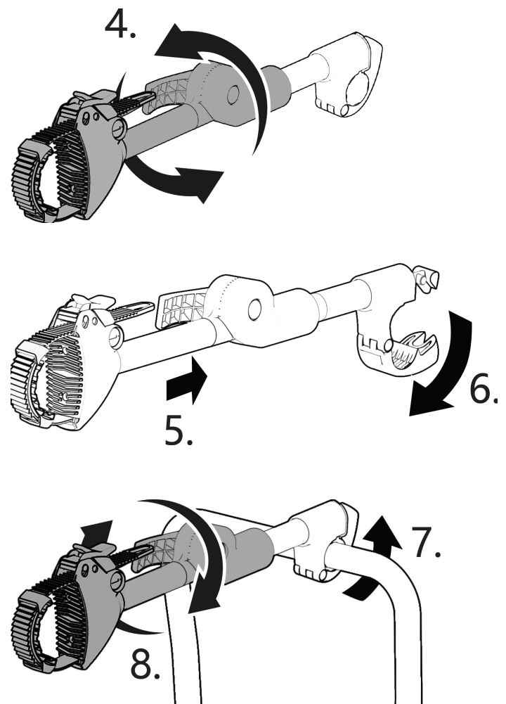
Figure 4: Mounting on U-bolt
