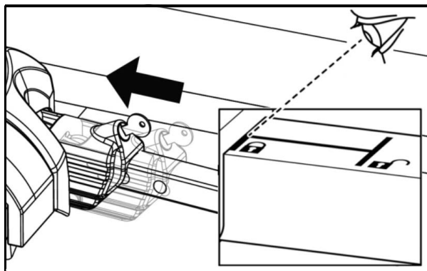
Figure 10: Locking the quick-release fastener
