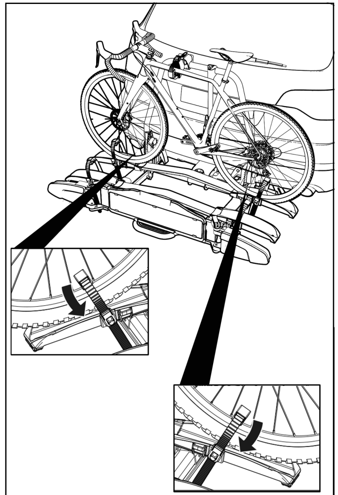
Figure 19: Attaching the wheels of the first bike
