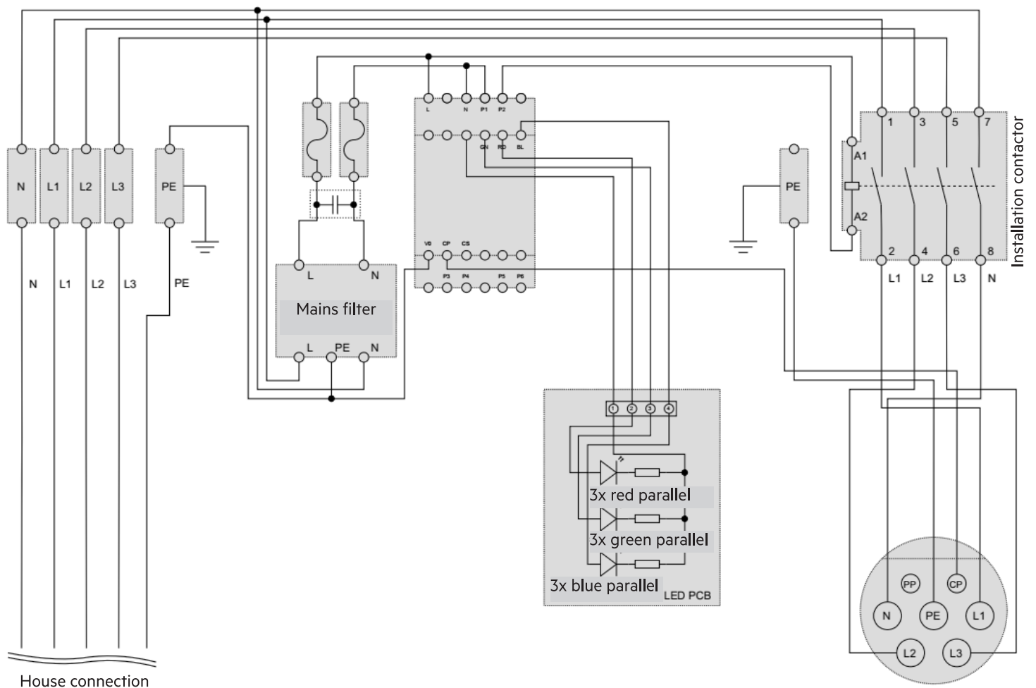
Fig. 4: Circuit diagram 11201, 11203
