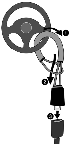
Figure 2: Montage
