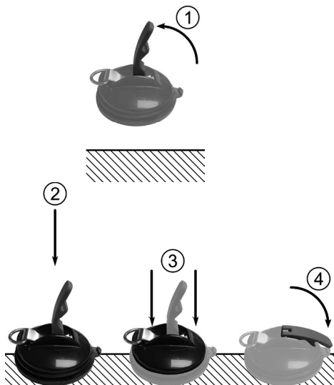
Picture 2: Mounting
