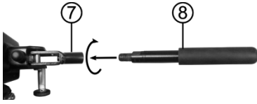
Figure 7: Mounting the tension lever
